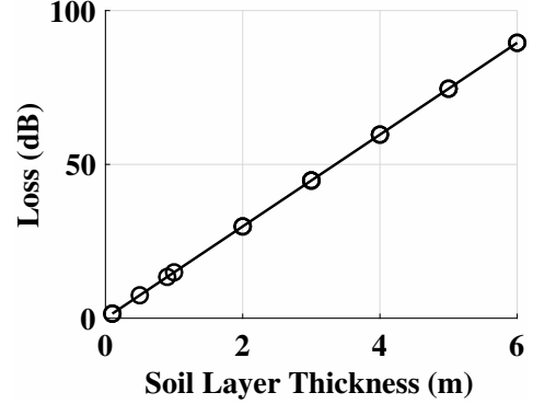
Fig. 6: The propagation loss in the soil medium with change in layer thickness.
